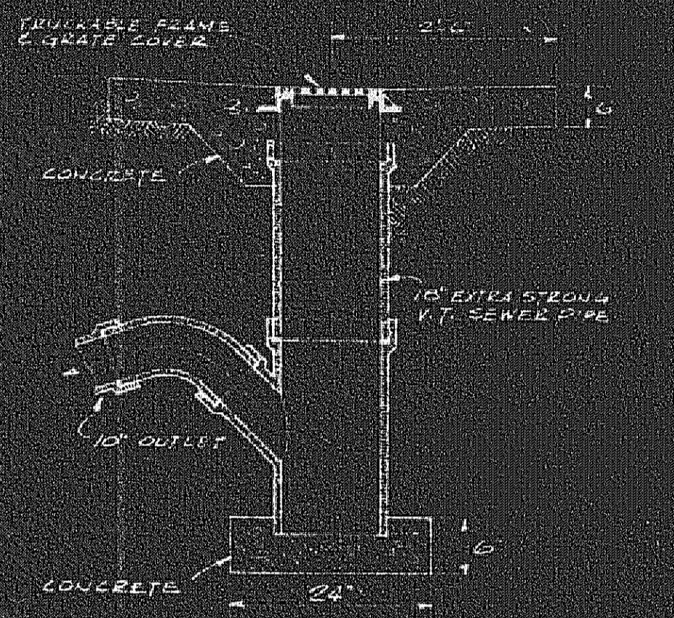
CATCH BASIN DETAIL NO SCALE
