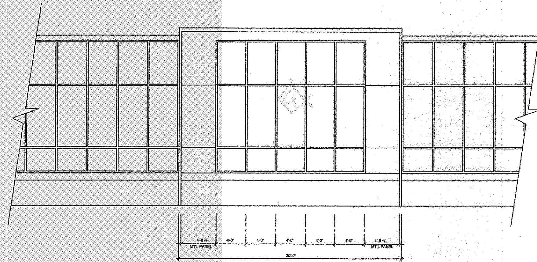
PARTIAL EAST ELEVATION SCALE: 1/8" = 1'-0"
