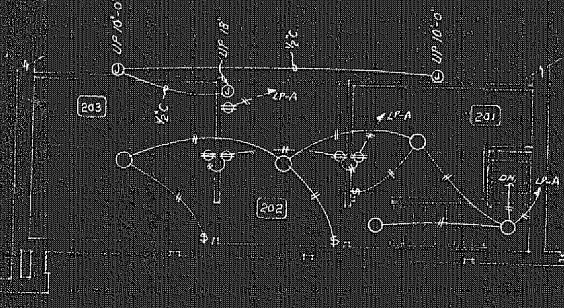
MEZZANINE ELECTRICAL PLAN SCALE 1/8" = 1'-0"
