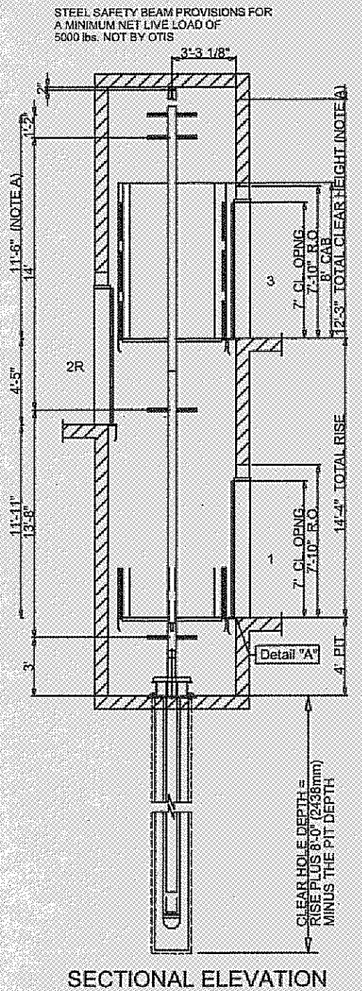
SECTIONAL ELEVATION
