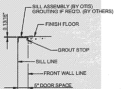
DETAIL "A" ADEQUATE SUPPORT AT ALL FASTENING POINTS OF ENTRANCE ASSEMBLY REQUIRED. (NOT BY OTIS)
